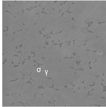
Figure 15: SEM at 50 \mu m from interface of AISI 321 LPWHT specimen
