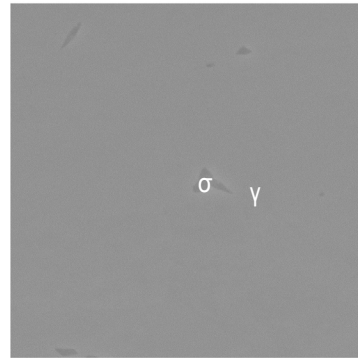
Figure 16: SEM at 3000 \mu m from interface of AISI 321 cladder LPWHT specimen
