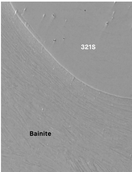
Figure 10: SEM of metallography of interface - As cladded specimen
