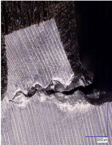
Figure 8: Optical micrographs of side profile of shear fracture, specimen head forming + LPWHT
