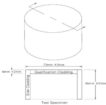
Figure 3: G146 Specimen Design
