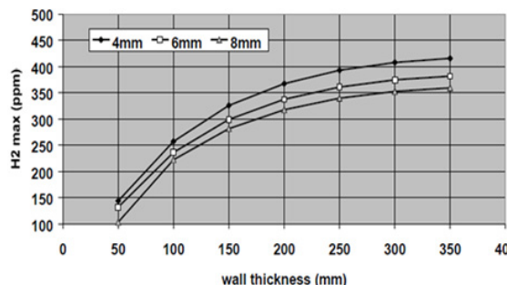
Figure 1: Influence of overlay thickness on hydrogen content at the interface
